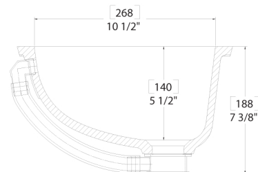
SIDE CROSS-SECTION
