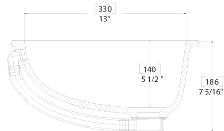
SIDE CROSS-SECTION
